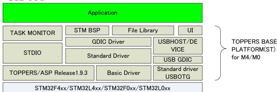
図 3.2.1 TOPPERS BASE PLATFORM(ST) for STM32F4xx/L4xx/F0xx/L0xx 構造図
